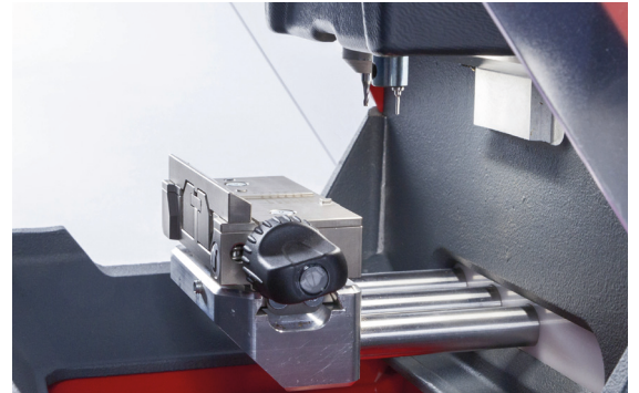
M Clamp Kit Residential/Commercial Part # OPZ11088B-BS
